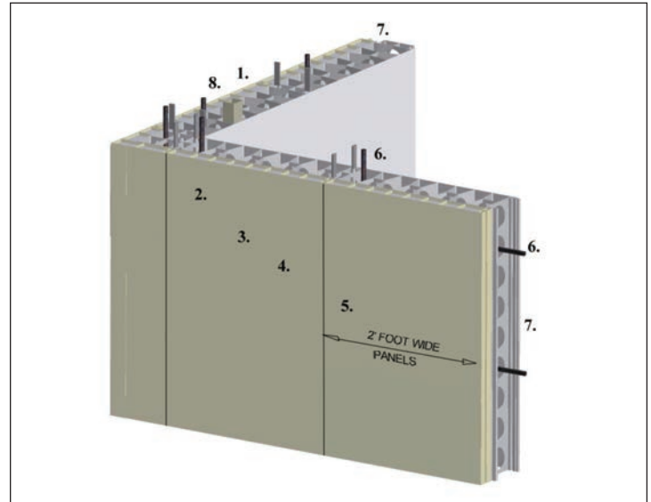
P624i - 6" THICK CONCRETE FORM PANEL WITH 2" INSULATION
