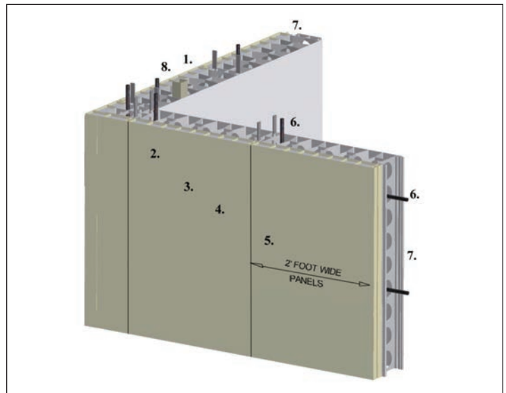
6" and 8" THICK CONCRETE FORM PANEL WITH 2" INSULATION
